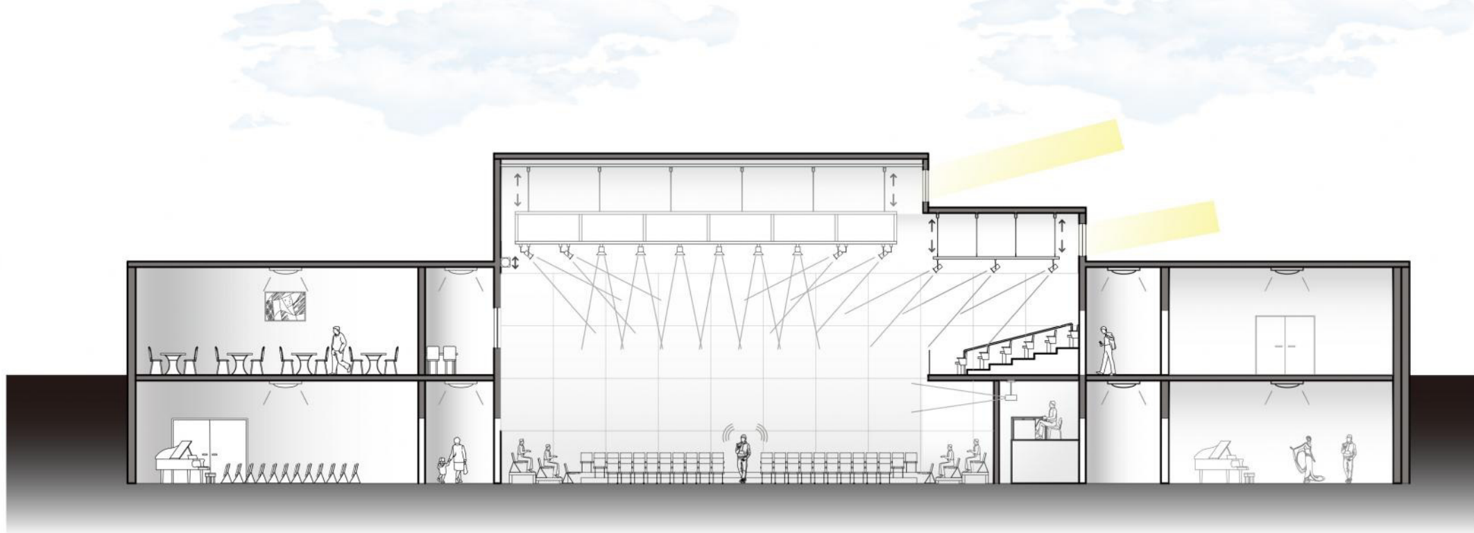
SECTION A - 'ARENA' OR 'THRUST' (1:200)
