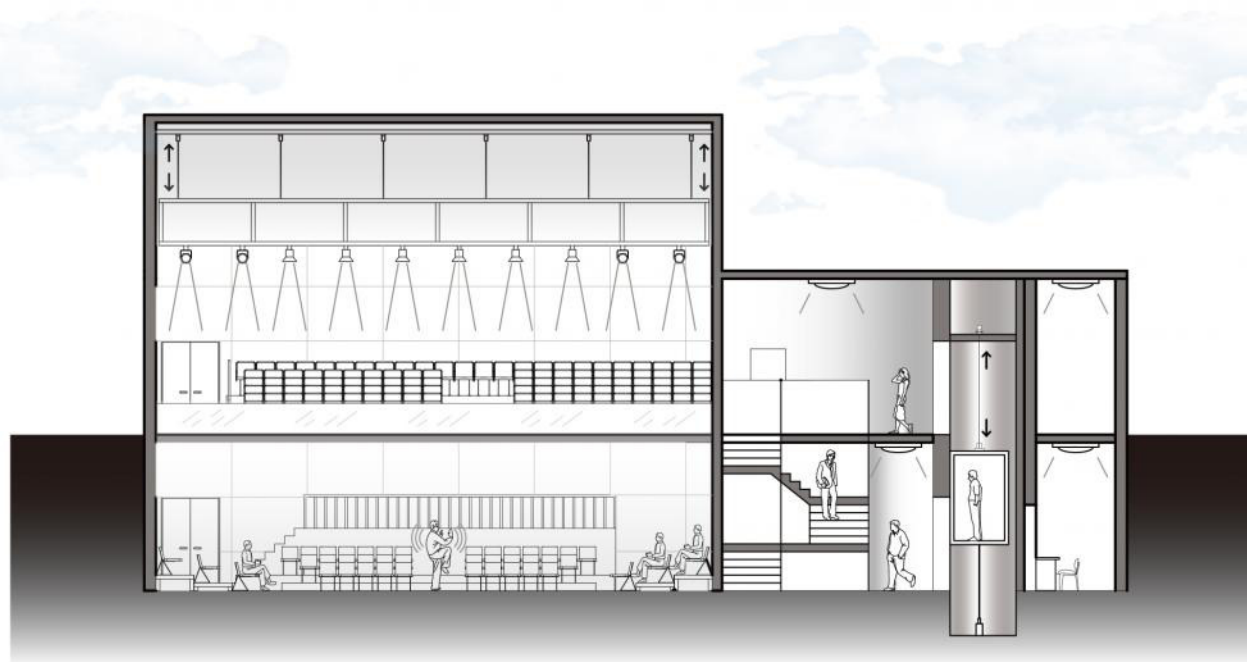
SECTION B - 'ARENA' OR 'THRUST' (1:200)
