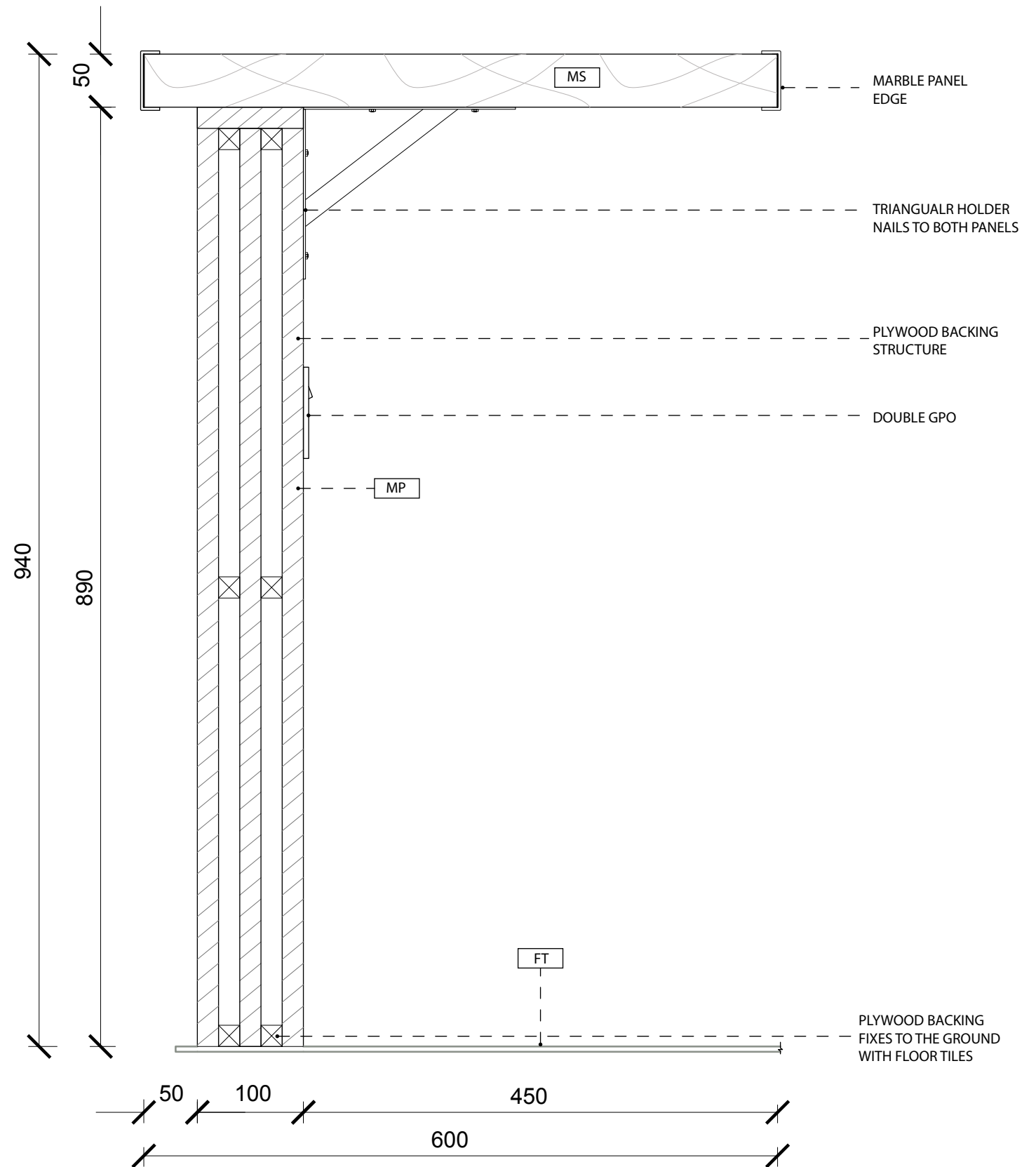
B A300 DETAILED SECTION 01 1:5
