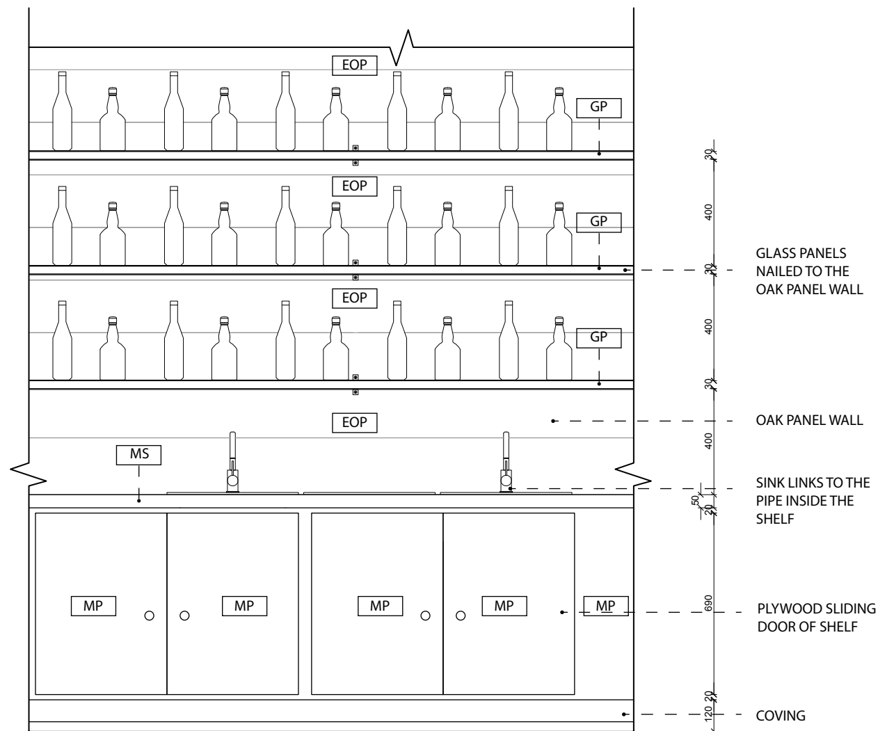
DETAILLED JOINERY 03 ELEVATION A A302 1:20
