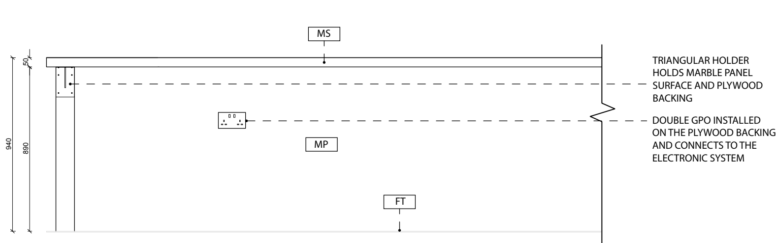
A A300 DETAILED JOINERY 01 ELEVATION 1:20
