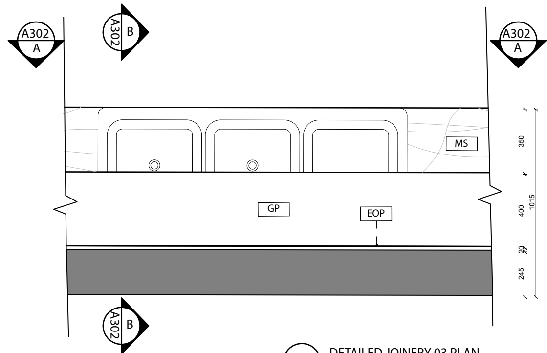
DETAILLED JOINERY 03 PLAN A302 1:20
