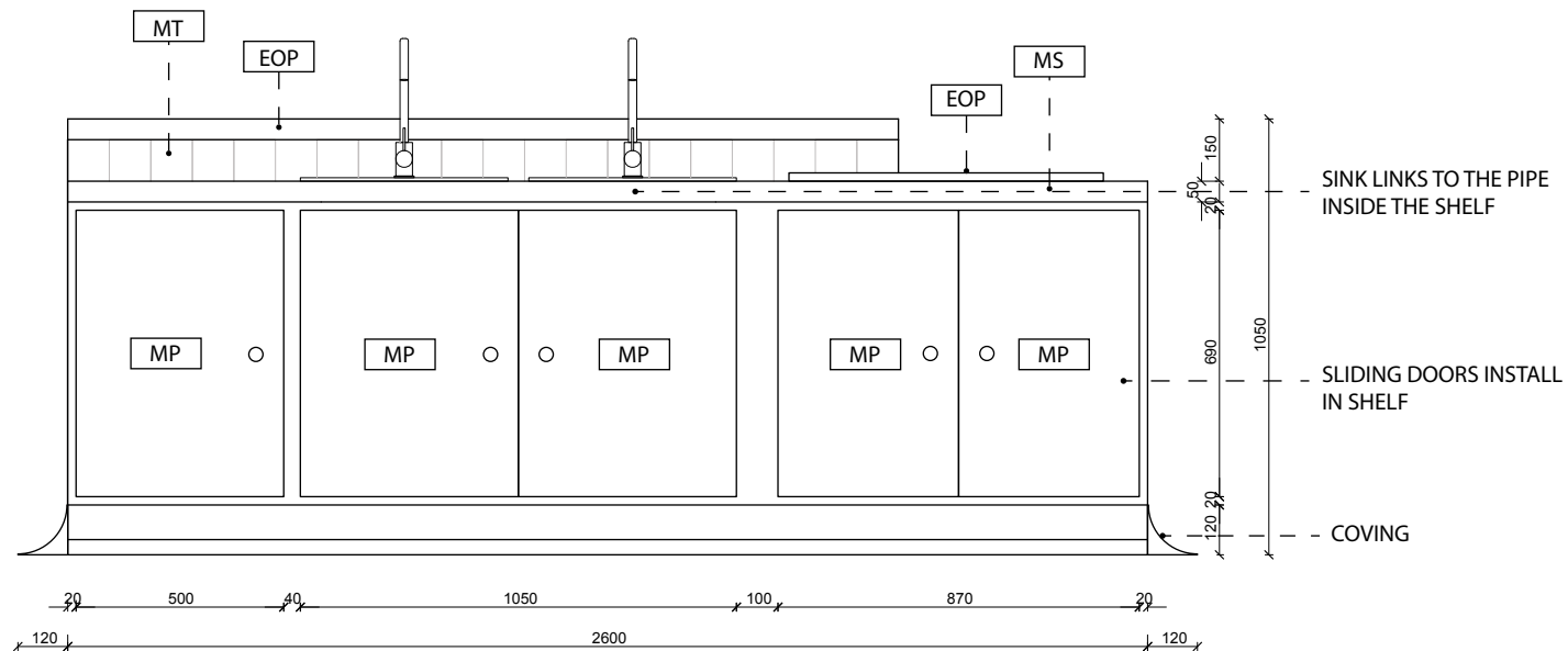
A A301 DETAILED JOINERY 02 ELEVATION 1:20
