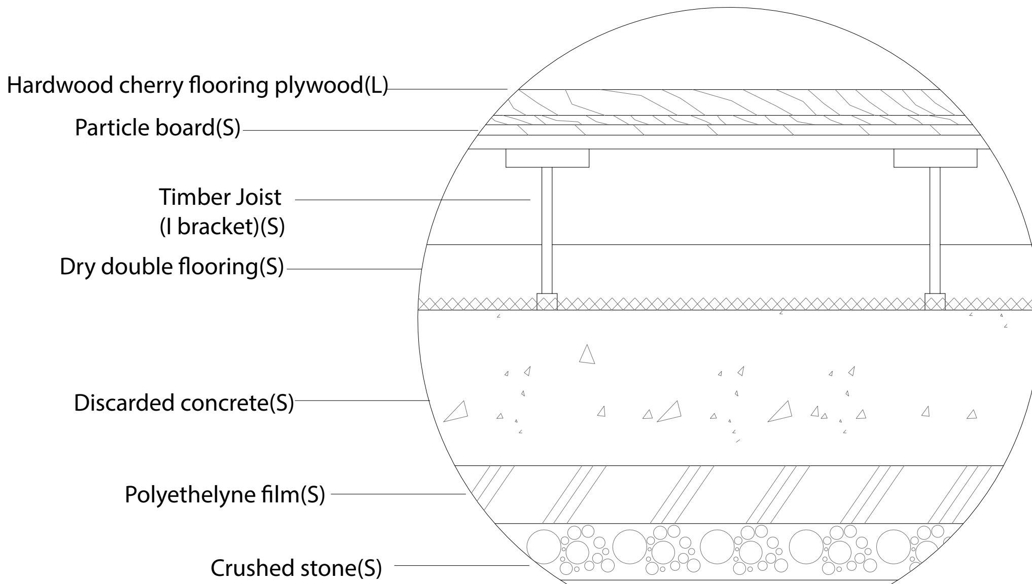
D. Underground construction detail
